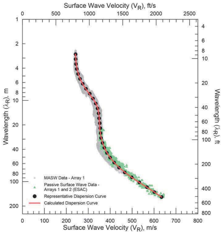
Arrays 1 and 2 - Field, representative and calculated surface wave dispersion data (left) and associated V_s model (right)
