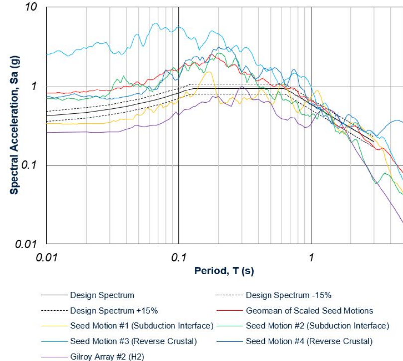
Scaled Pseudo-Spectral Acceleration Response Spectra from GM Selection with the Design Spectrum
