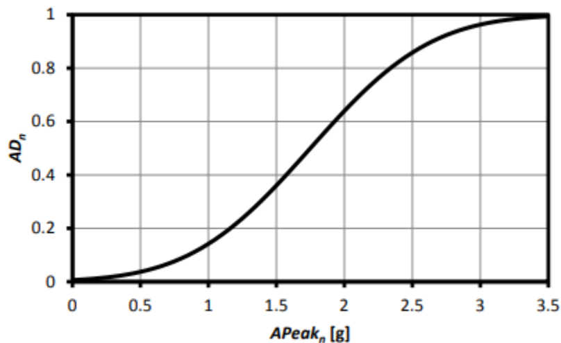
Figure 3: Function relating peak roof acceleration, APeak_n , and equipment damage as a percentage of equipment cost ( AD_n )
