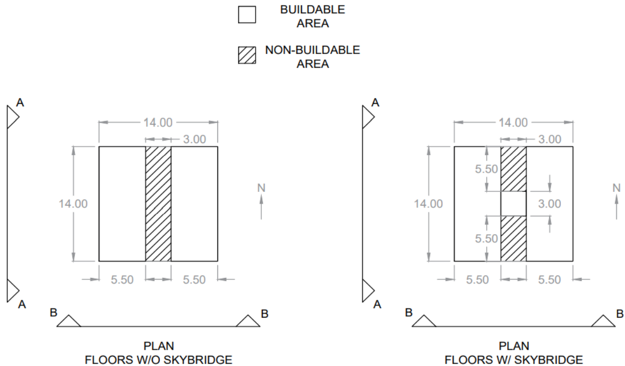
Figure 1: Buildable floor areas for (a) floors without a skybridge and (b) floors with a skybridge. no members can be placed within the hatched area.
