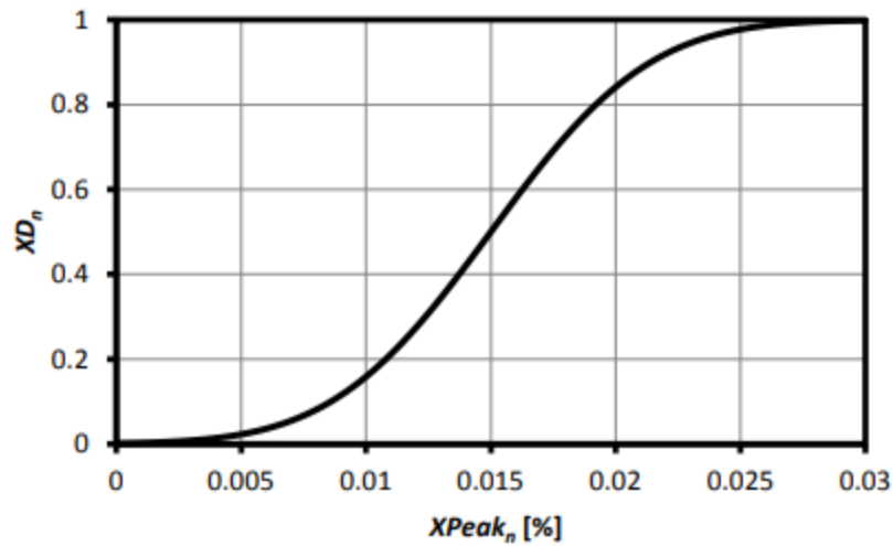
Figure 2: Function relating peak roof drift, XPeak_n , and structural damage as a percentage of construction cost ( XD_n )
