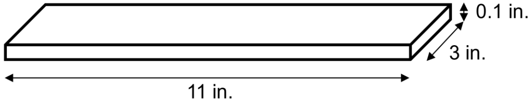
Figure 5 Maximum dimensions for wall members.
