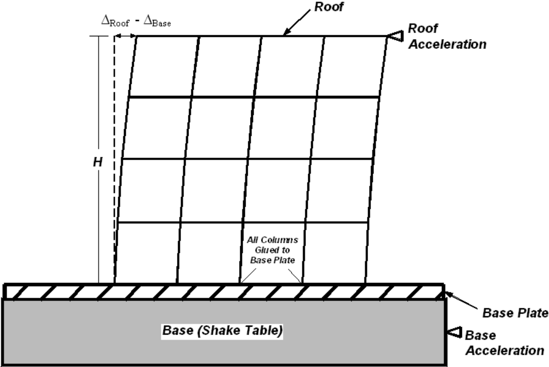
Figure 18 Typical set-up of model shakedown.
