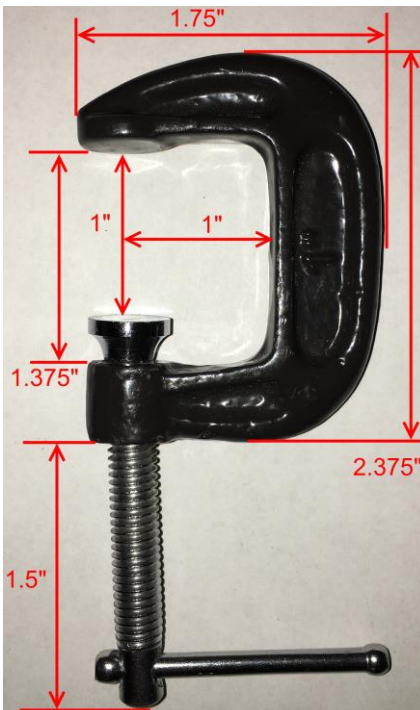
Figure 17 Location of roof accelerometer and dimensions of c-clamps used to secure roof accelerometer (1" = 2.54 cm).
