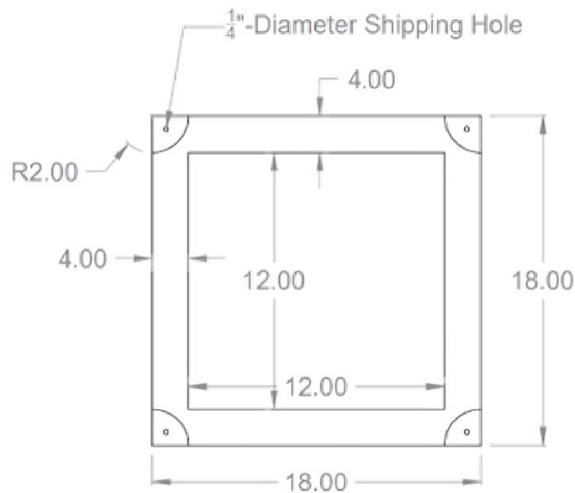
Figure 12 Typical base plate for model.
