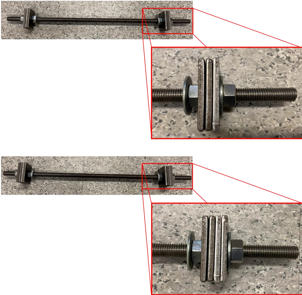
Figure 16 (TOP) Dead weight configuration for a typical floor. (BOTTOM) Dead weight configuration on the highest relevant floor.
