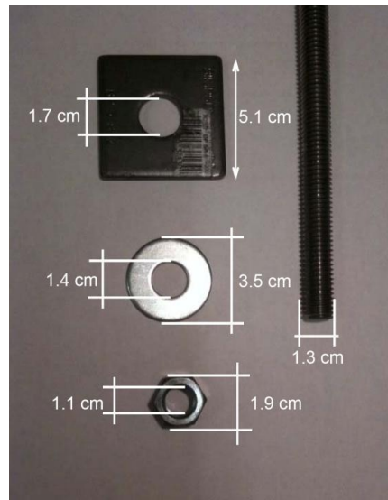
Figure 15 Dimensions of dead-weight components used throughout structure (1 in = 2.54 cm).
