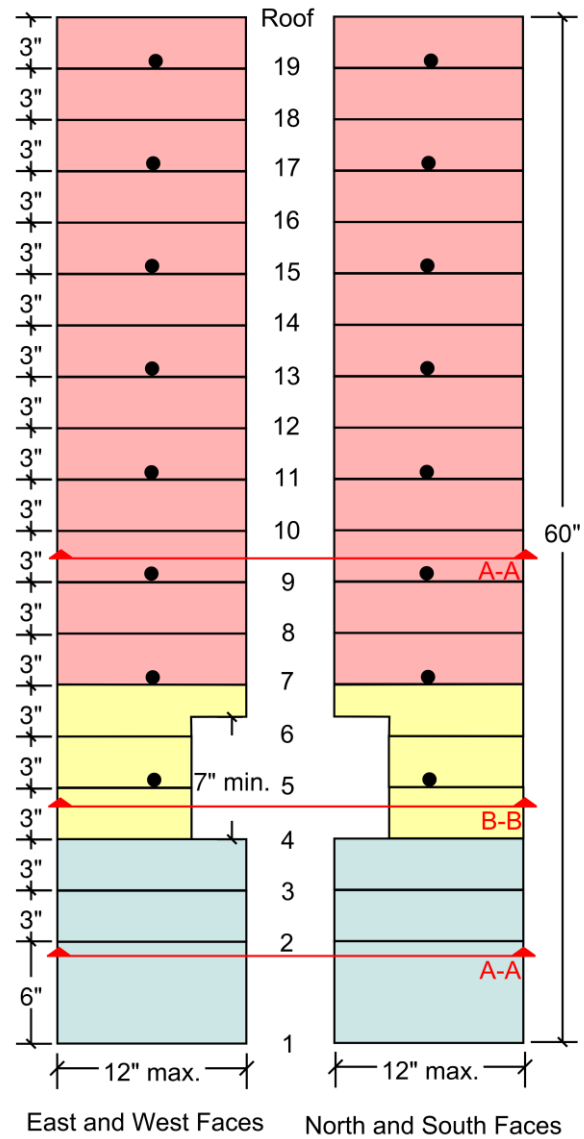
Figure 2 Illustration of building zones in the structural model for f = 19 . Refer to Figure 1 for notation used in elevation views. Black-filled circles represent the location of dead loads for shake-table testing. Note that building envelope is mirror-symmetrical about its diagonals
