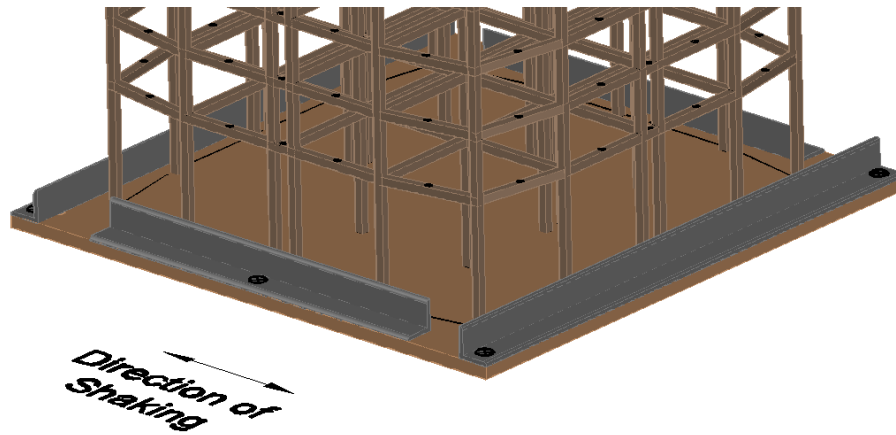
Figure 14 Typical attachment of base plate to the shake table.
